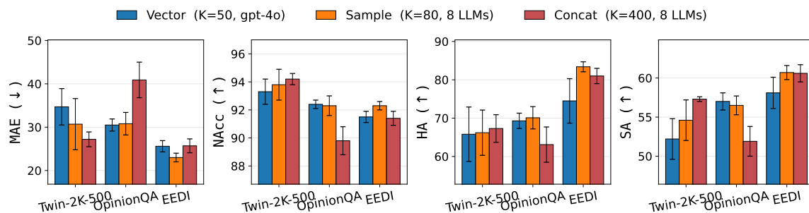
Figure C4: Population-level effect of broadening the LLM-side input over 5 seeds. The legend entries are Vector ( K=50 ), Sample ( K=80 ), and Concat ( K=400 ).
