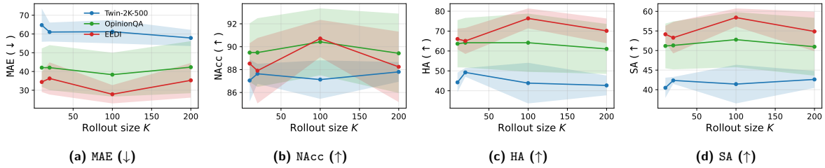
Figure C5: Population-level metrics as a function of single-source rollout size K . Each curve is the mean across 5 seeds with shaded \pm 1 s.d. Source is fixed to gpt-4o and the head matches Vector of Table 1. Legend shown only in panel (a) and shared across panels.
