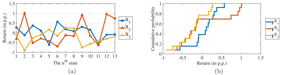
Figure 1: Three risky returns and their cumulative mass functions
