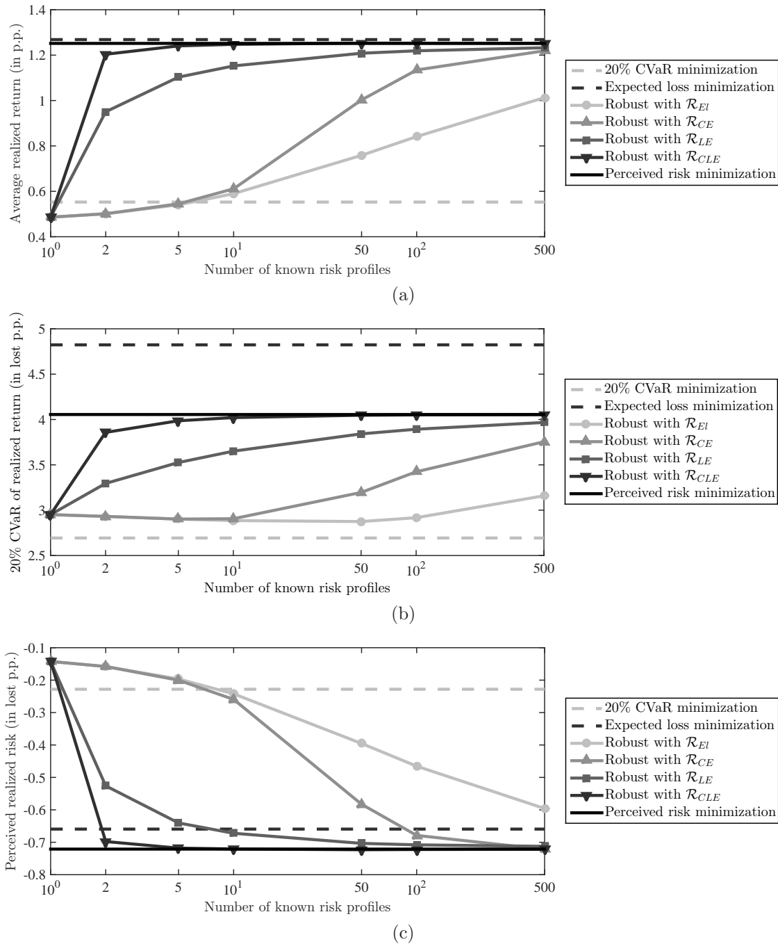
Figure 3: Statistic about the out of sample performance of the portfolios proposed by the different methods when implementing them on the week following the analysis. (a) compares the average return over the 5000 experiments. (b) compares the 20% CVaR of the empirical distribution described by the returns obtained in the 5000 experiments. (c) presents the risk as perceived by the investor for this distribution.
