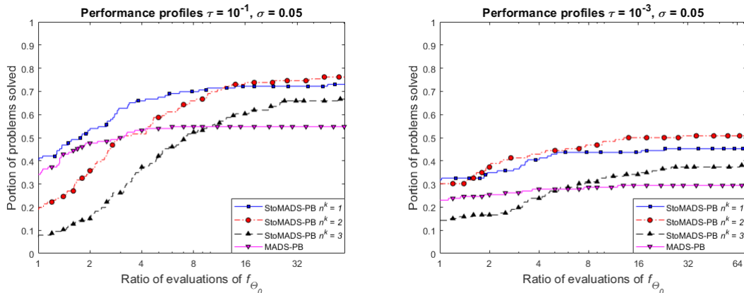
Figure 7: Performance profiles for convergence tolerances \tau = 10^{-1} and \tau = 10^{-3} , and noise level \sigma = 0.05 on 126 analytical constrained test problems additively perturbed in the intervals I(\sigma, x^0, f) and I(\sigma, x^0, c_j) .
