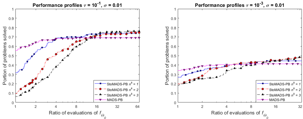
Figure 3: Performance profiles for convergence tolerances \tau = 10^{-1} and \tau = 10^{-3} , and noise level \sigma = 0.01 on 126 analytical constrained test problems additively perturbed in the intervals I(\sigma, x^0, f) and I(\sigma, x^0, c_j) .
