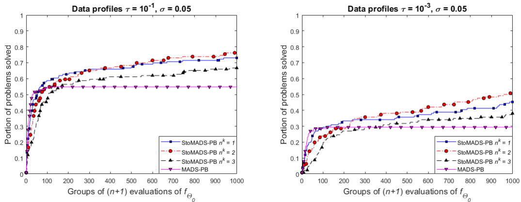
Figure 6: Data profiles for convergence tolerances \tau = 10^{-1} and \tau = 10^{-3} , and noise level \sigma = 0.05 on 126 analytical constrained test problems additively perturbed in the intervals I(\sigma, x^0, f) and I(\sigma, x^0, c_j) .
