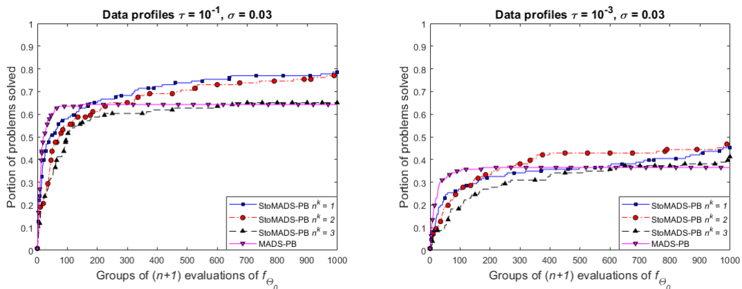
Figure 4: Data profiles for convergence tolerances \tau = 10^{-1} and \tau = 10^{-3} , and noise level \sigma = 0.03 on 126 analytical constrained test problems additively perturbed in the intervals I(\sigma, x^0, f) and I(\sigma, x^0, c_j) .
