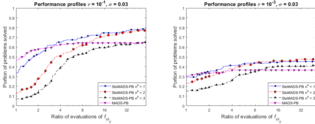
Figure 5: Performance profiles for convergence tolerances \tau = 10^{-1} and \tau = 10^{-3} , and noise level \sigma = 0.03 on 126 analytical constrained test problems additively perturbed in the intervals I(\sigma, x^0, f) and I(\sigma, x^0, c_j) .
