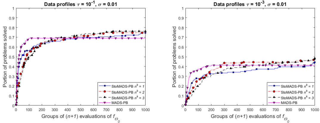
Figure 2: Data profiles for convergence tolerances \tau = 10^{-1} and \tau = 10^{-3} , and noise level \sigma = 0.01 on 126 analytical constrained test problems additively perturbed in the intervals I(\sigma, x^0, f) and I(\sigma, x^0, c_j) .
