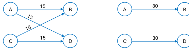
Figure 2: Illustration of alternative grouping strategies for pattern repetition
