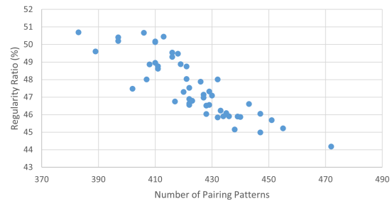
Figure 4: Dispersion of regularity ratio vs. number of pairing patterns across 50 initial solutions (2019 Dataset)
