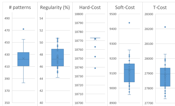
Figure 3: Distribution of 50 solutions generated by the initial crew pairing optimizer across key indicators (2019 Dataset)
