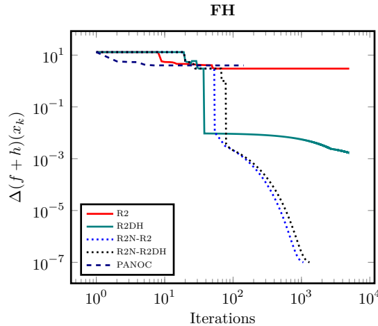
Figure 4: FH objective vs. iterations.
