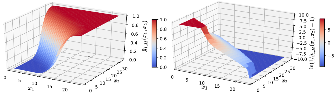
Figure 2: 3D surface plots of \hat{g}_{1,M}(x_1, x_2) and \ln(1/\hat{g}_{1,M}(x_1, x_2) - 1)
