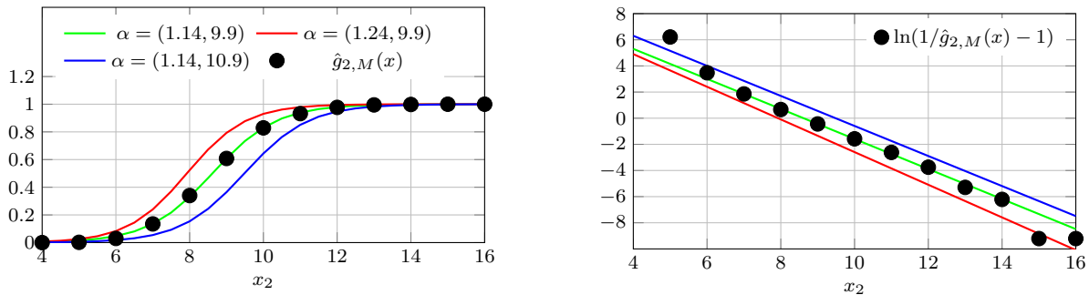
Figure 1: Fitting \hat{g}_{2,M}(x) with logistic and \ln(1/\hat{g}_{2,M}(x) - 1) with linear functions
