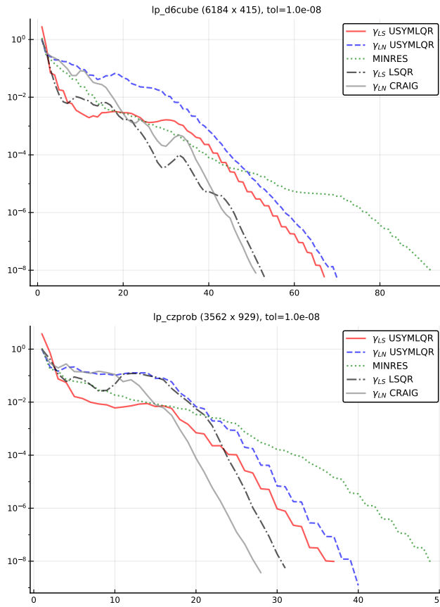
Figure 2: Convergence curves on under-determined problems from the SuiteSparse Matrix Collection. The horizontal axis represents iterations. In red and blue are the backward errors (40) and (42), respectively, along the usymqr iterations. The green dotted curve is the backward error (43) for (4) along the minres iterations. The black dash-dotted curve is the backward error (40) along lsqr iterations, while the gray curve is the backward error (42) along the craig iterations.
