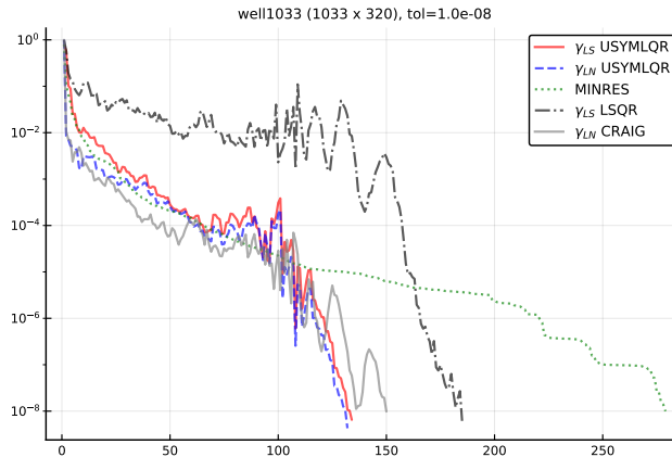
Figure 3: Convergence curves on an over-determined problems from the SuiteSparse Matrix Collection. The horizontal axis represents iterations. In red and blue are the backward errors (40) and (42), respectively, along the usymqlr iterations. The green dotted curve is the backward error (43) for (4) along the minres iterations. The black dash-dotted curve is the backward error (40) along lsqr iterations, while the gray curve is the backward error (42) along the craig iterations.
