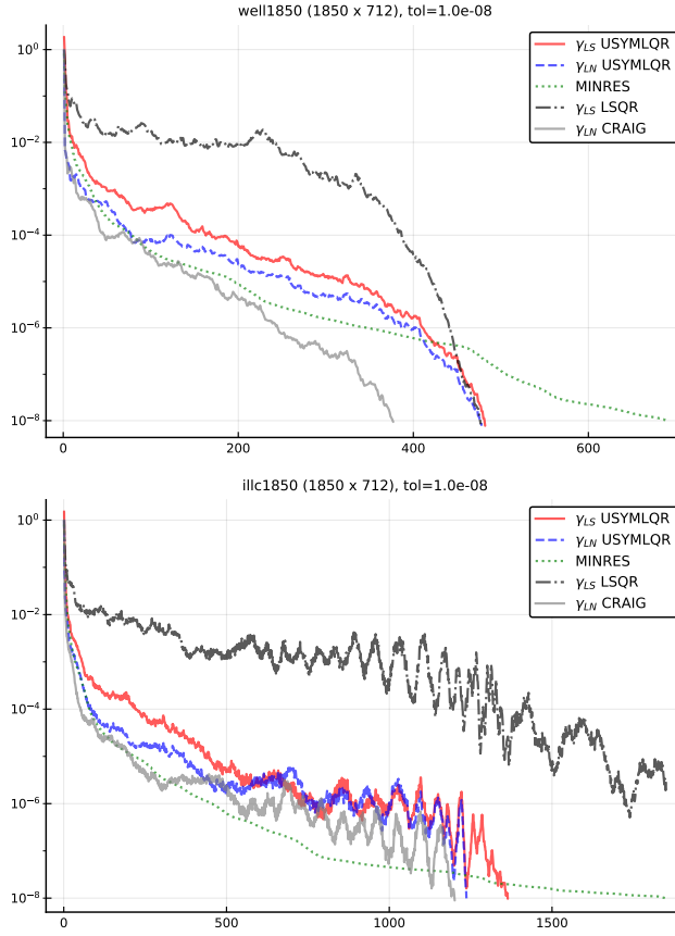
Figure 1: Convergence curves on under-determined problems from the SuiteSparse Matrix Collection. The horizontal axis represents iterations. In red and blue are the backward errors (40) and (42), respectively, along the usymqlr iterations. The green dotted curve is the backward error (43) for (4) along the minres iterations. The black dash-dotted curve is the backward error (40) along lsqr iterations, while the gray curve is the backward error (42) along the craig iterations.
