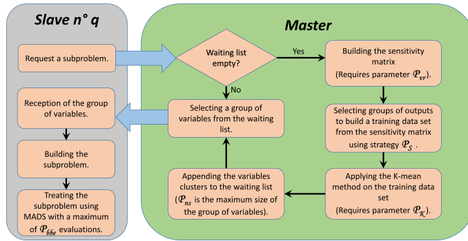
Figure 3: The process of selecting a group of variables for a regular slave.
