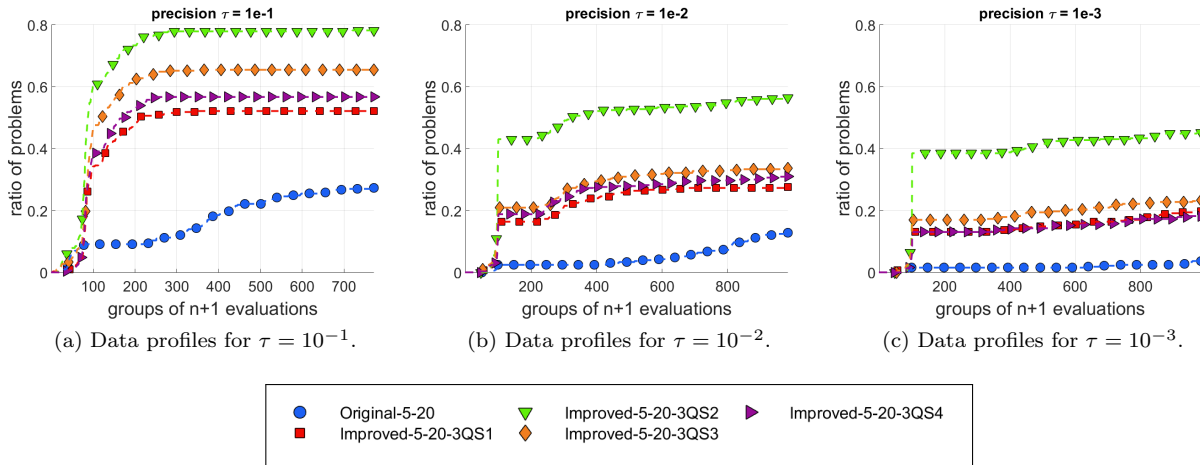
Figure 6: Comparison of methods with different strategies \mathcal{P}_{vr} for regrouping outputs.
