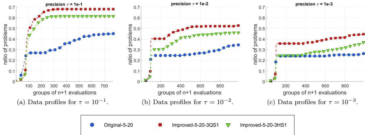
Figure 5: Comparison of the improved methods with different ranges of the parameter k for the k -mean algorithm ( \mathcal{P}_K ).
