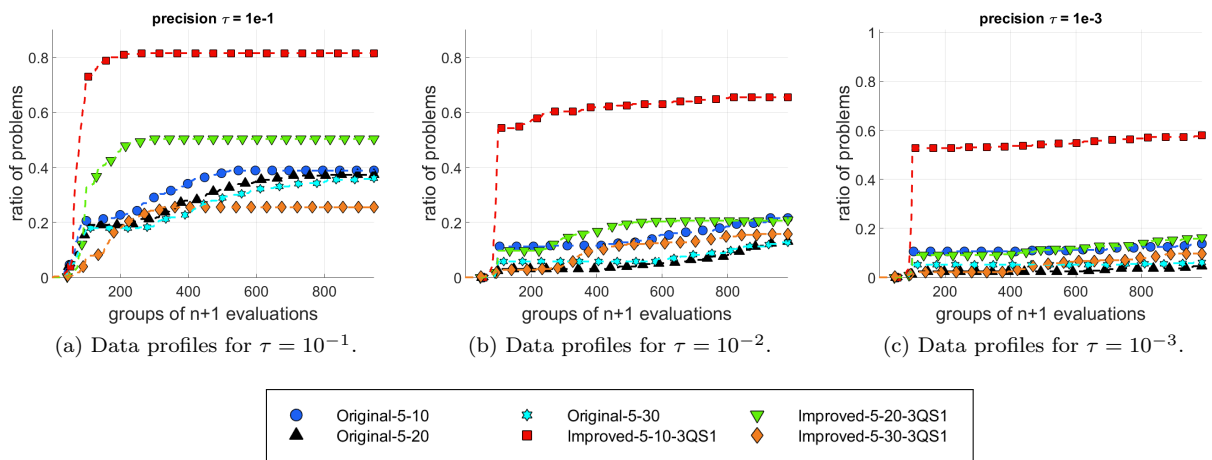
Figure 8: Selecting a default value of the maximum blackbox evaluations \mathcal{P}_{bbe} for the subproblems in PSD-MADS.
