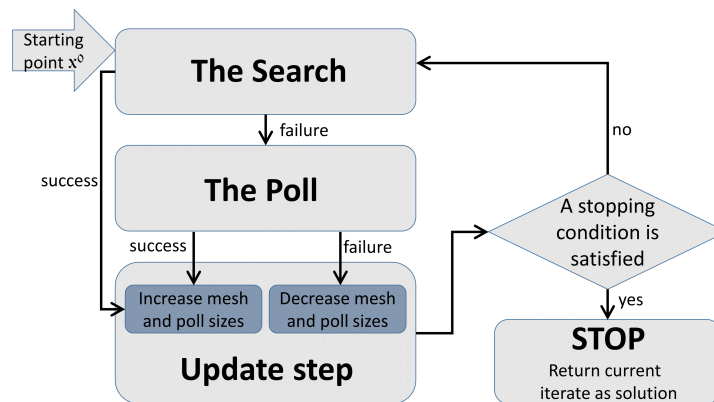
Figure 1: Overview of the MADS algorithm (Figure adapted from [2]).
