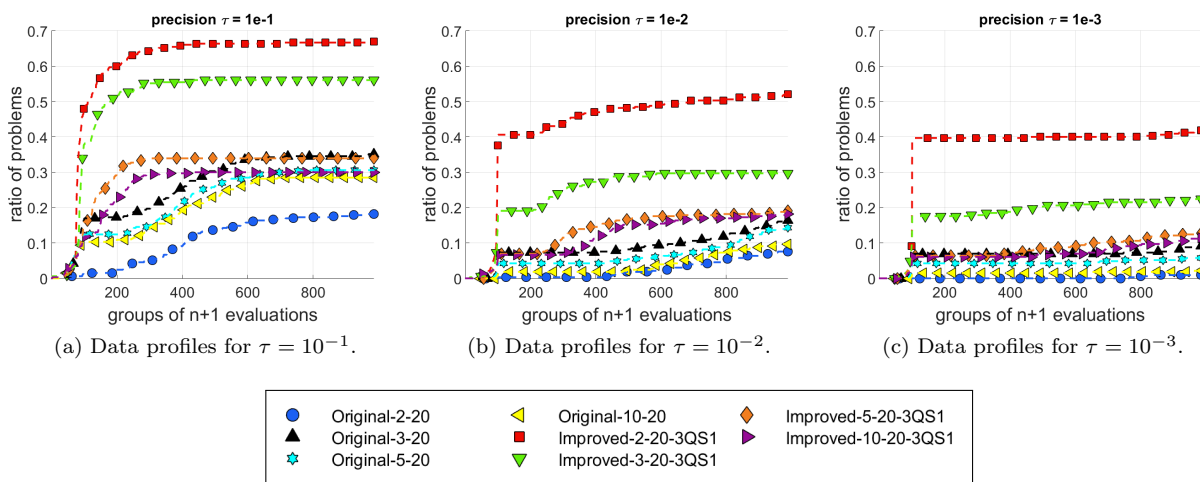
Figure 7: Selecting a default value of the upper bound on the subproblem size \mathcal{P}_{ns} for the improved version of PSD-MADS.
