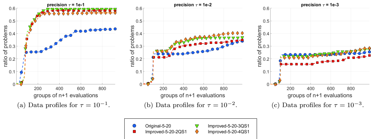
Figure 4: Comparison of the original and improved methods with different number of variable ranges 10^{\mathcal{P}_{vr}} for building the sensitivity matrix.
