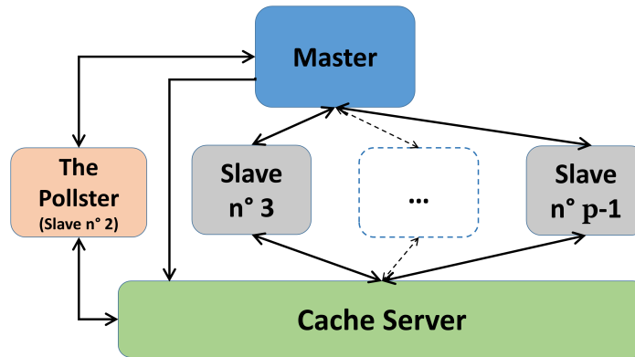
Figure 2: The interactions between the p different processes in PSD-MADS.
