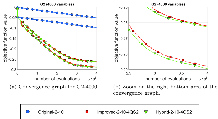
Figure 10: Convergence graph of the best and the worst runs of each algorithm with problem G2-4000.
