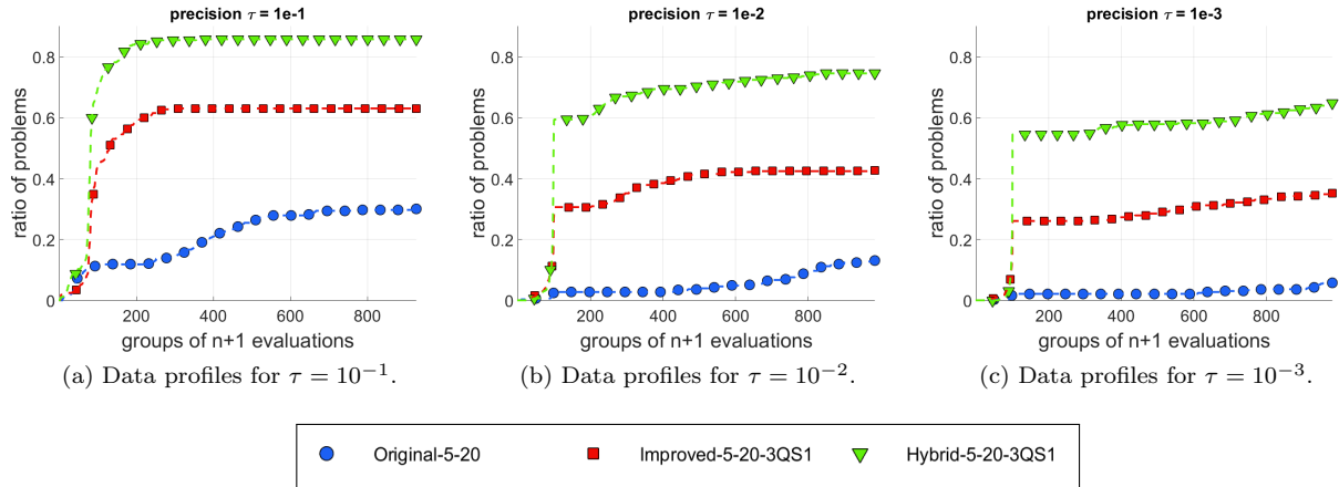
Figure 9: Comparing the hybrid method to the original and improved PSD-MADS.
