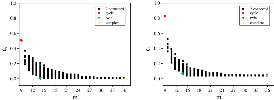
(a) The vertex residual mean distance, \varepsilon_v , versus the number of edges for all 2-connected graphs on 9 vertices. Highlighted are the cycle, the complete graph, and the twin graphs.
