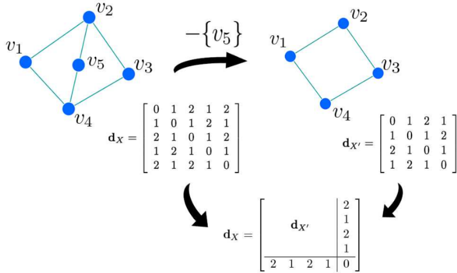
Figure 1: For a k -GC graph X and v \in V(X) let X' = X \setminus v . The matrix d_{X'} is a submatrix of the matrix d_X .
