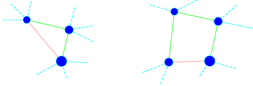
(a) Triangle in an arbitrary graph. The existence of a triangle given any 3 vertices has as consequence the minimal impact by edge failure, increasing the Wiener index by 1 when the failure occurs.
