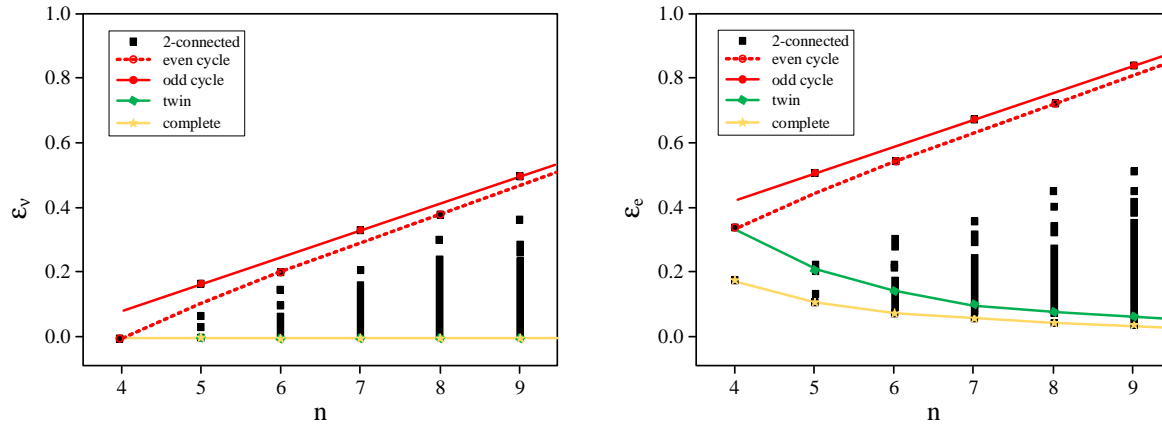
(a) The vertex residual mean distance, \varepsilon_v , versus the number of vertices for all 2-connected graphs from 4 up to 9 vertices. Highlighted in red are the graphs maximizing \varepsilon_v , i.e. the cycle graphs (Equation 3), and in yellow-green the graphs minimizing \varepsilon_v , i.e. the complete graphs (Equation 1), and the twin graphs (Equation 5).
