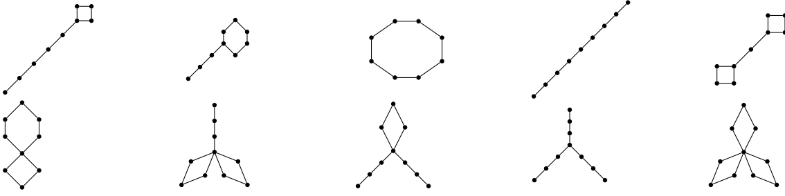
Figure 3: Graphs H_1, \dots, H_{10} from Conjecture 1.
