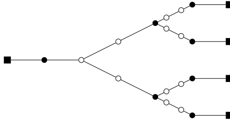
Figure 8: A peculiar critical tree which is not special, where a minimum dominating set contains vertices indicated by filled circles and leaves are indicated by squares.
