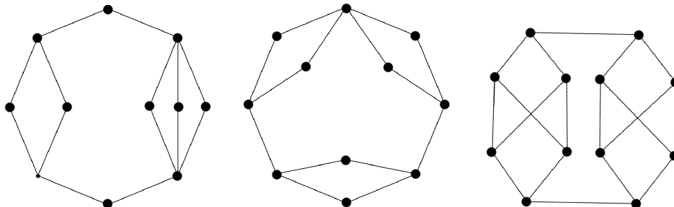
Figure 1: Examples of graphs with \eta + 2r \leq n + 2 and \eta + D < n .
