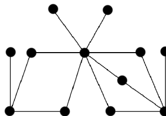
Figure 2: A graph with D + \eta + \omega = n + 2 ( n = 12 , \omega = 2 , \eta = 6 and D = 6 ).
