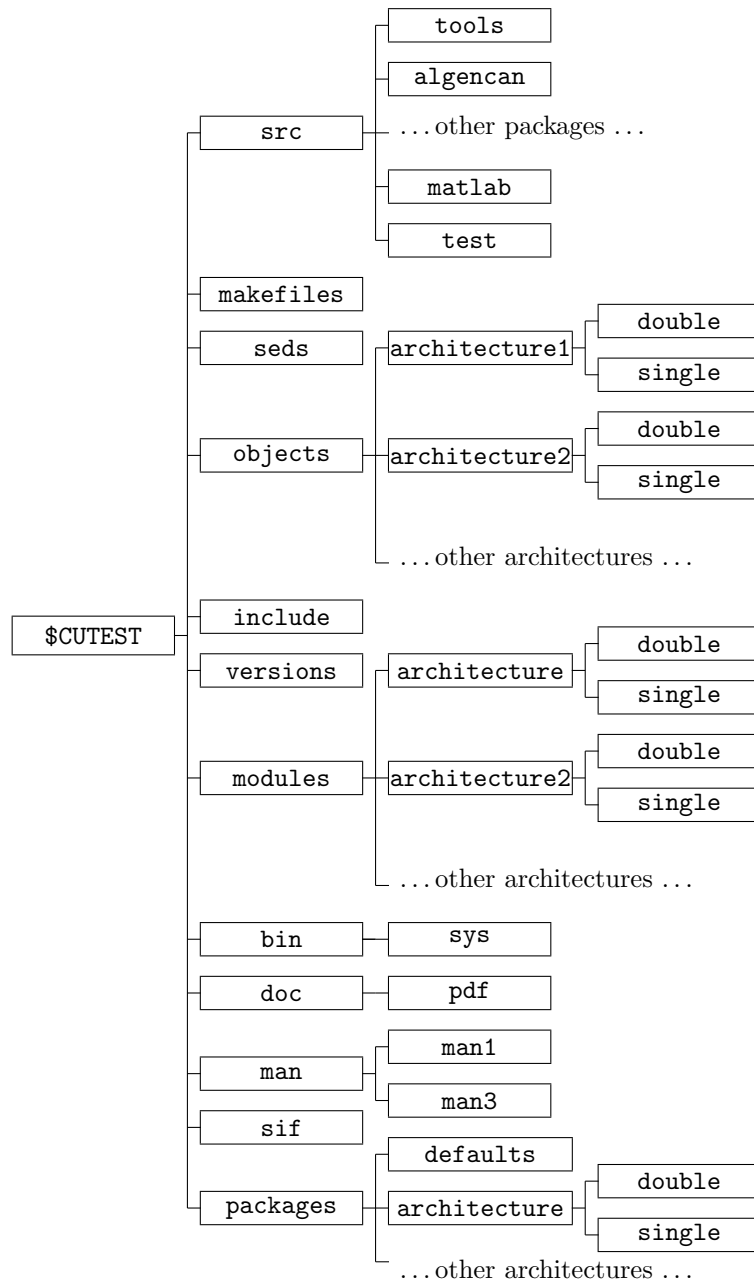
Figure 1: Structure of the CUTEst directories
