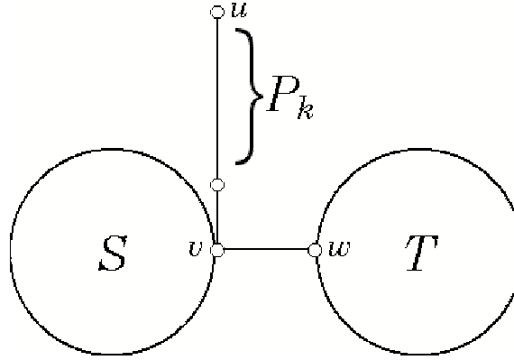
Figure 1: The structure of G .
