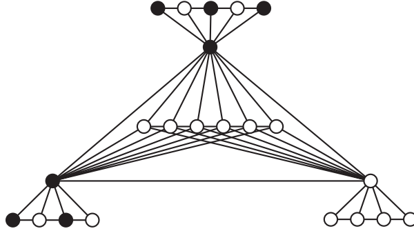
Figure 3. Extremal graph for n = 22 .
