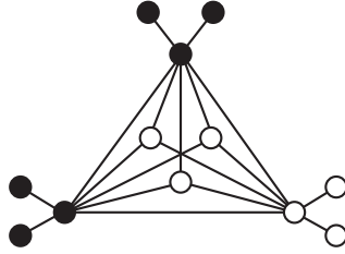
Figure 4. Extremal graph for n = 12 .
