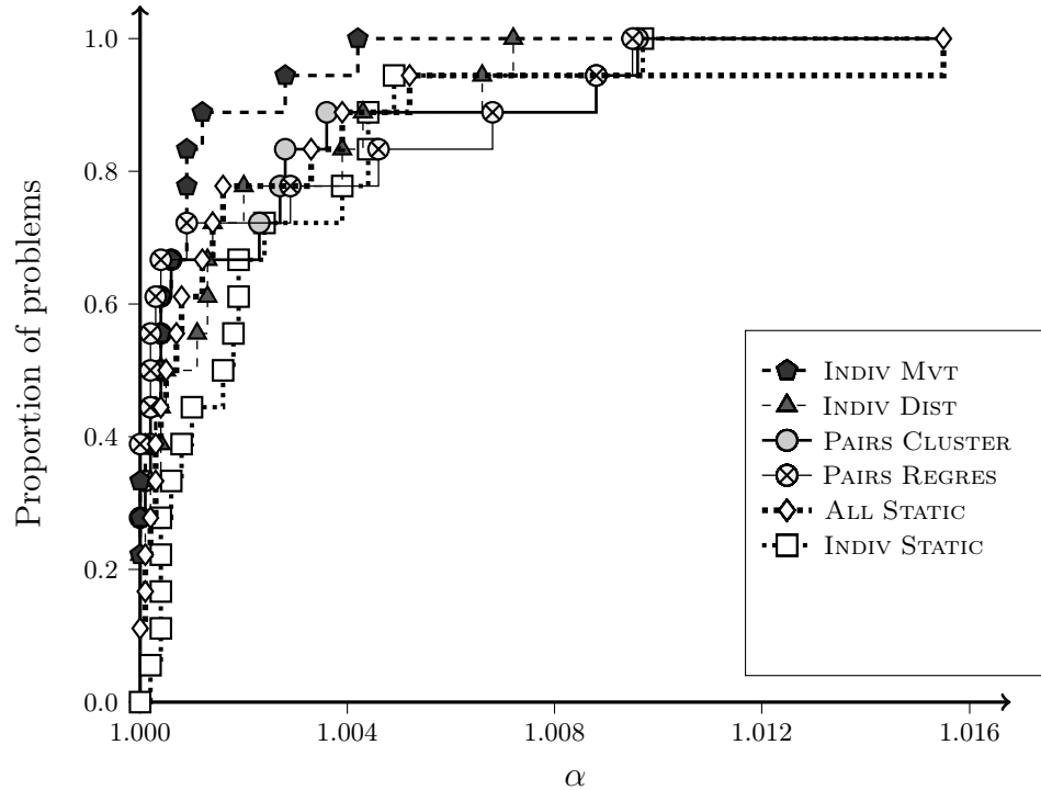
Figure 4: Performance profile [21] for the six selected algorithms applied to the 18 instances using the true objective.
